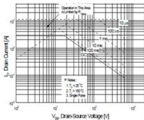
Figure 9-3. Maximum Safe Operating Area for T0251, T0252
