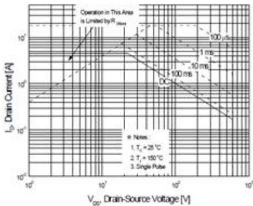
Figure 9-1. Maximum Safe Operating Area for T0220
