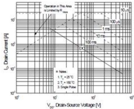
Figure 9-2. Maximum Safe Operating Area for T0220F
