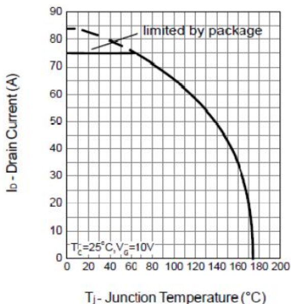
Drain Current
